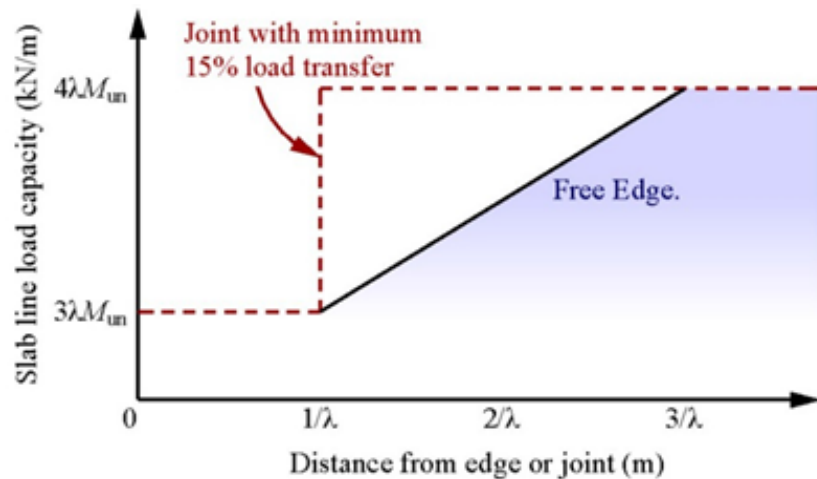
Figure 4-5: Line load capacity near free edges or joints from TR34 4 th edition
