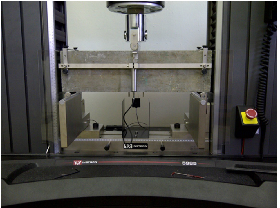
Figure 2-7: Beam test setup to EN 14651 with CMOD gauge and additional LVDT for displacement measurement.
