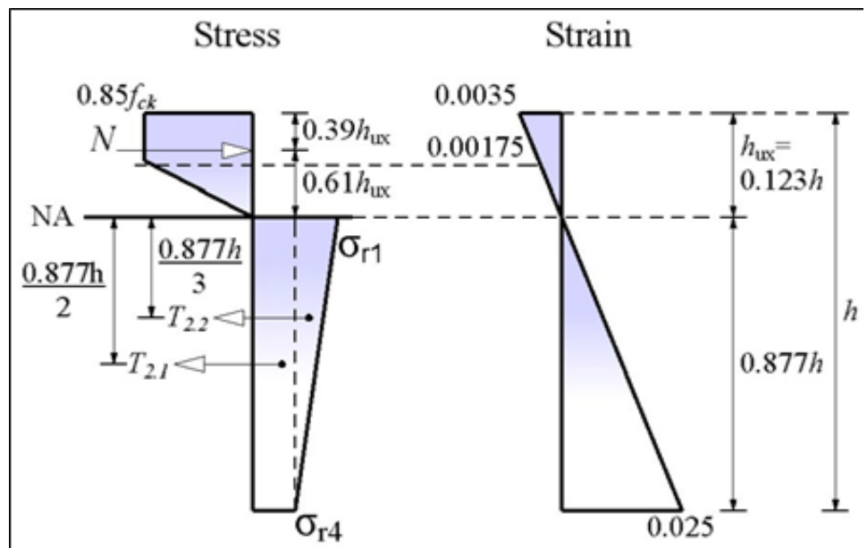
Figure 4-2: Stress block for fibre reinforced concrete
