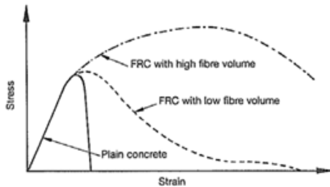
Figure 2-1: Toughness performance of fibre reinforced concrete
