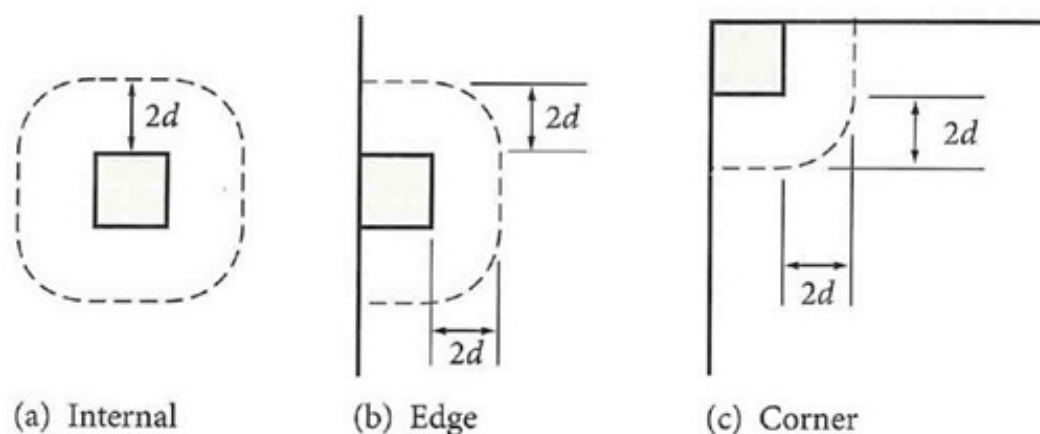
Figure 4-4: Critical perimeters for punching shear for internal, edge and corner loading
