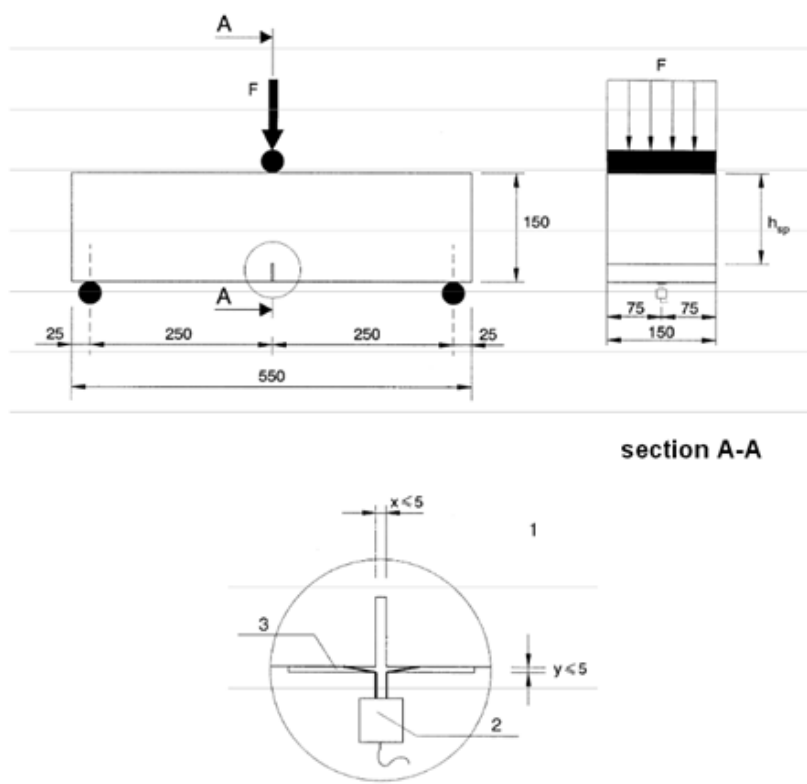
Figure 2-6: Three-point notched beam test setup from EN 14651 (2005)
