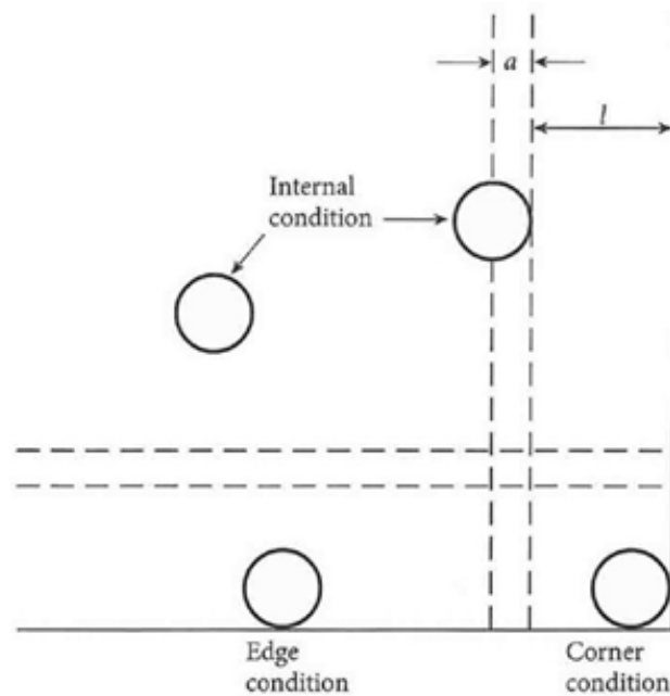
Figure 4-3: Definitions of loading conditions
