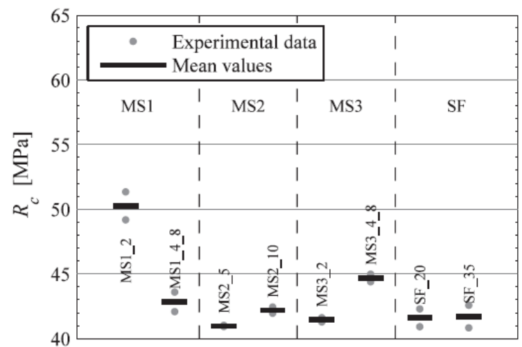
Figure 2-4: Relative performance of macro synthetic fibres and steel fibres in concrete compression.
