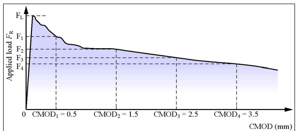
Figure 4-1: Example of Load vs. CMOD plot derived from EN14651 beam test (European Committee for Standardisation (CEN), 2005).
